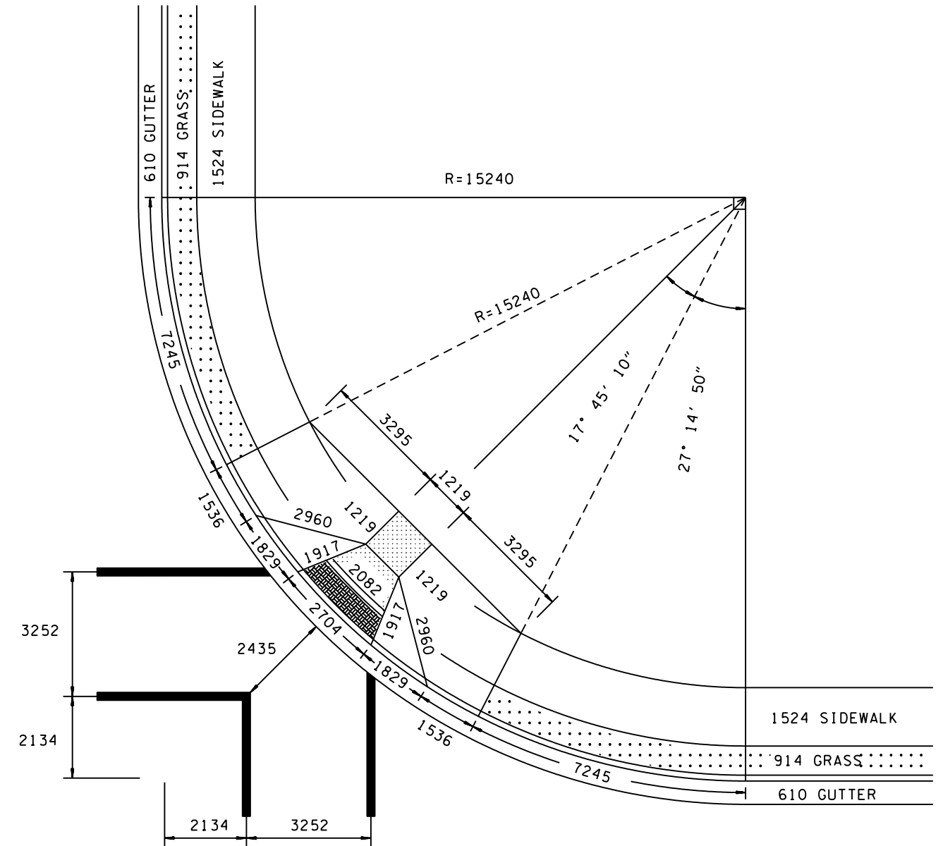
WITH 914 mm GRASS STRIP R=15240
