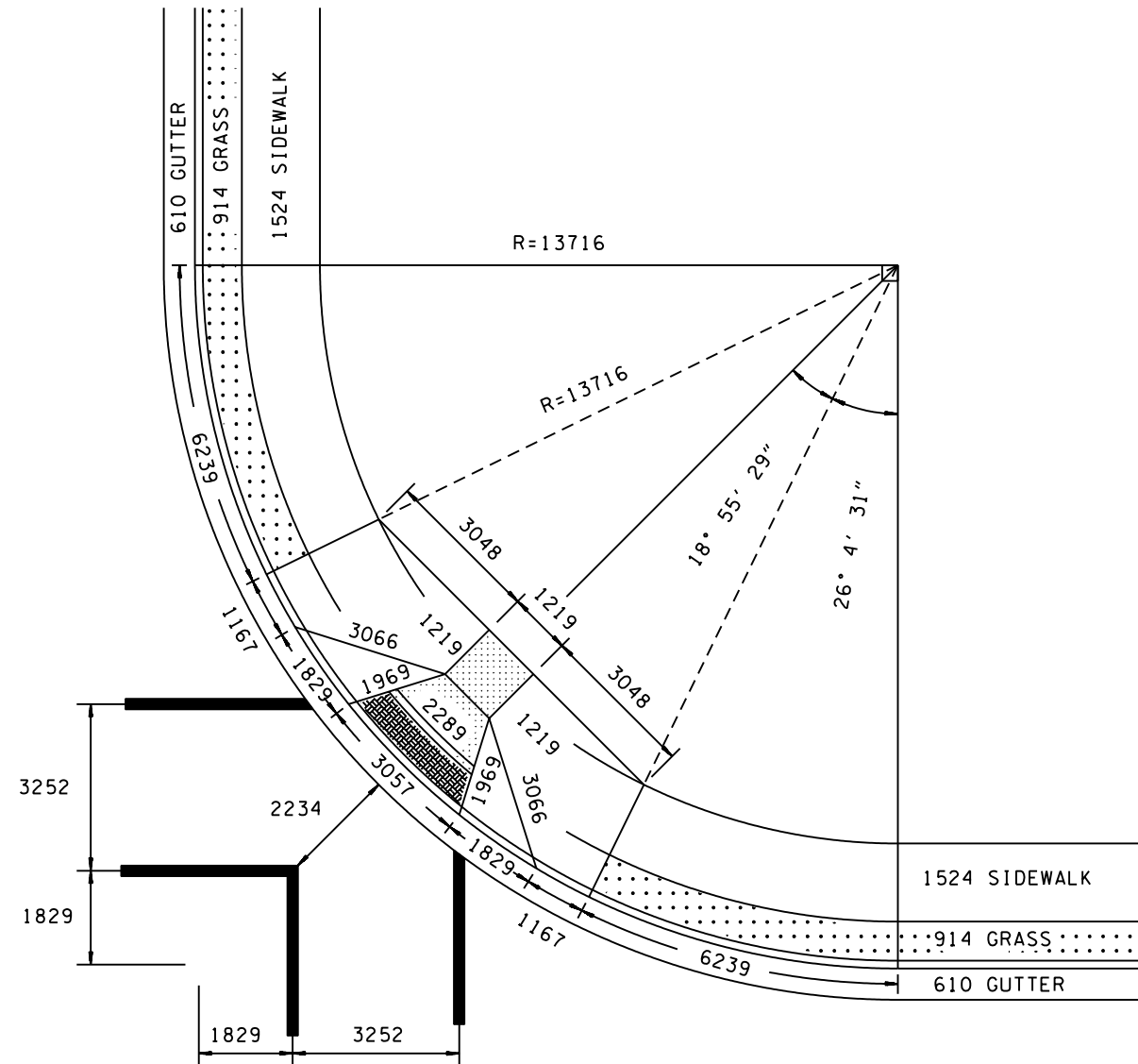
WITH 914 mm GRASS STRIP R=13716
